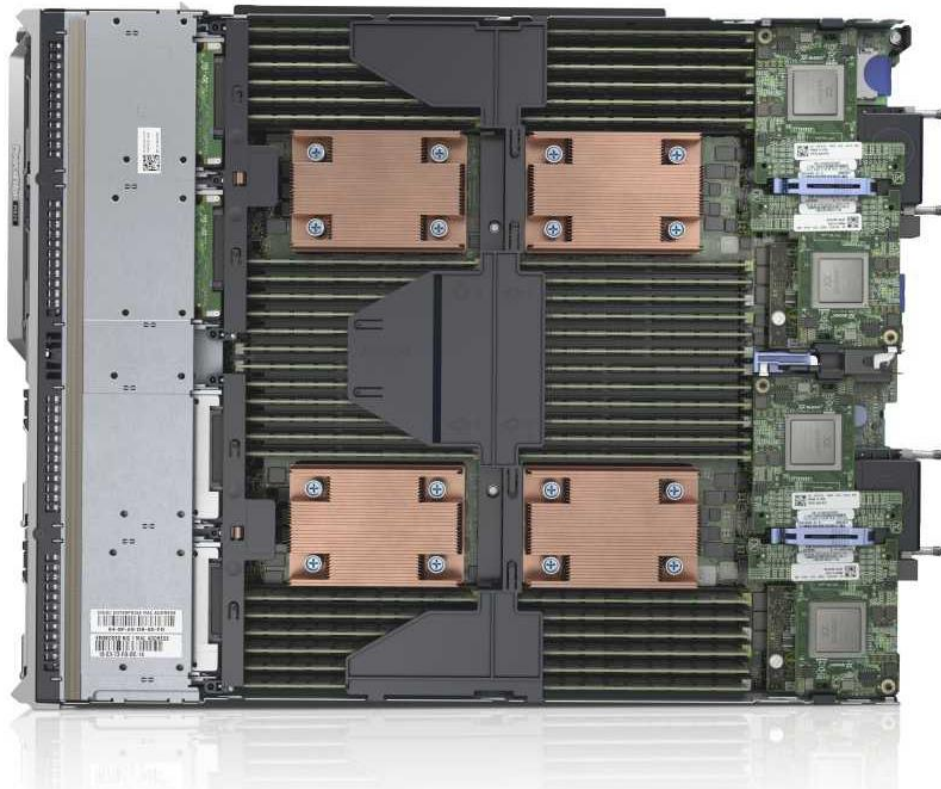
Figure 3. M820 internal module view
