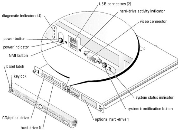
Figure 1-1. Front-Panel Features
