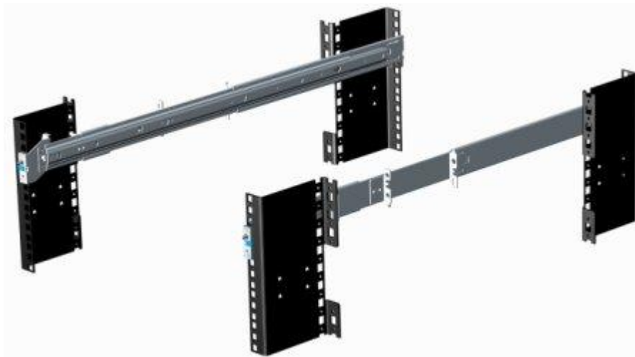
Figure 21. R510 Static Rails in Rack
