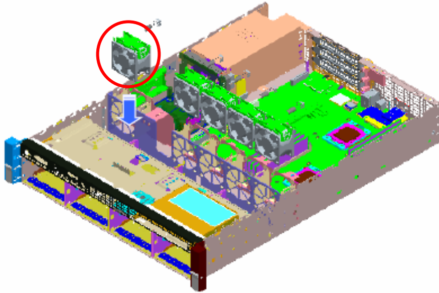
Figure 24. Fan Location
