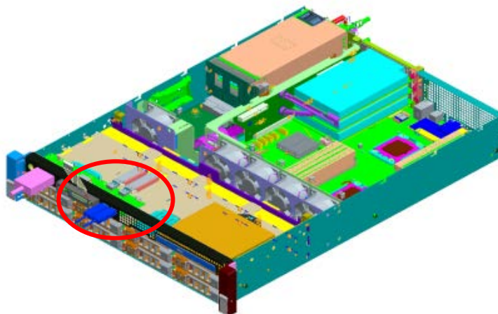
Figure 27. PowerEdge R510-8 Internal USB Connector
