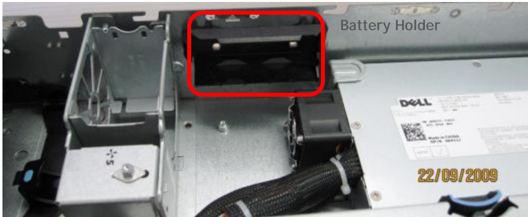
Figure 14. PowerEdge R510-4: Non-Redundant PSU and the Battery Holder for PERC Card
