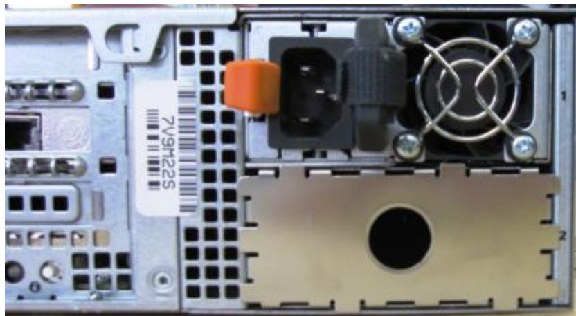
Figure 10. Non-redundant Power Supply Option on PowerEdge R510-8 and 12
