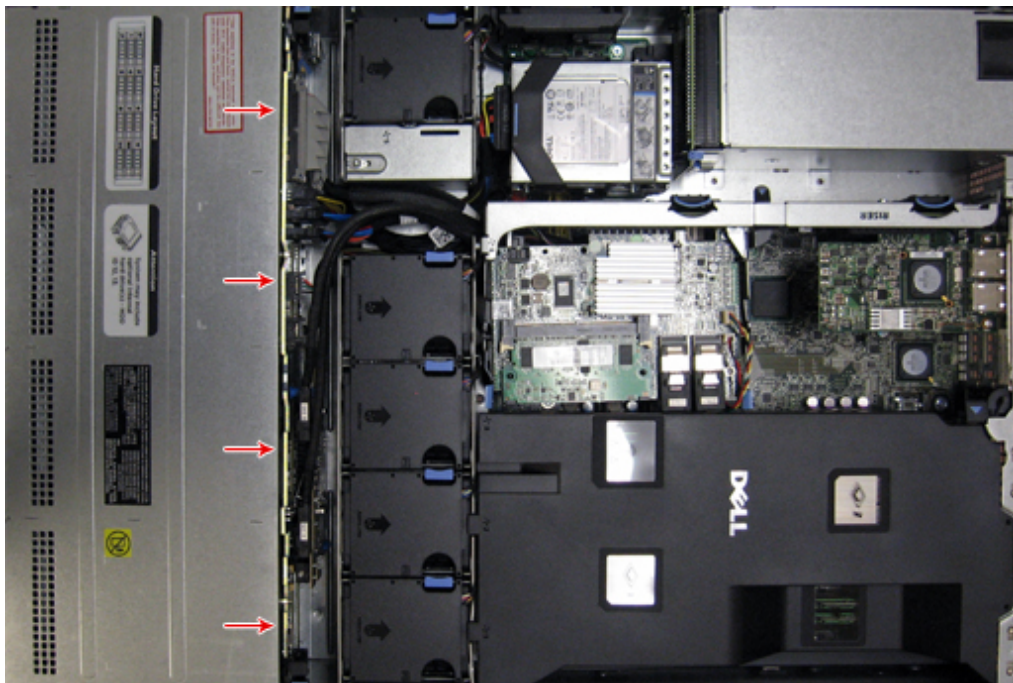
Figure 17. PowerEdge R510-12 Internal View
