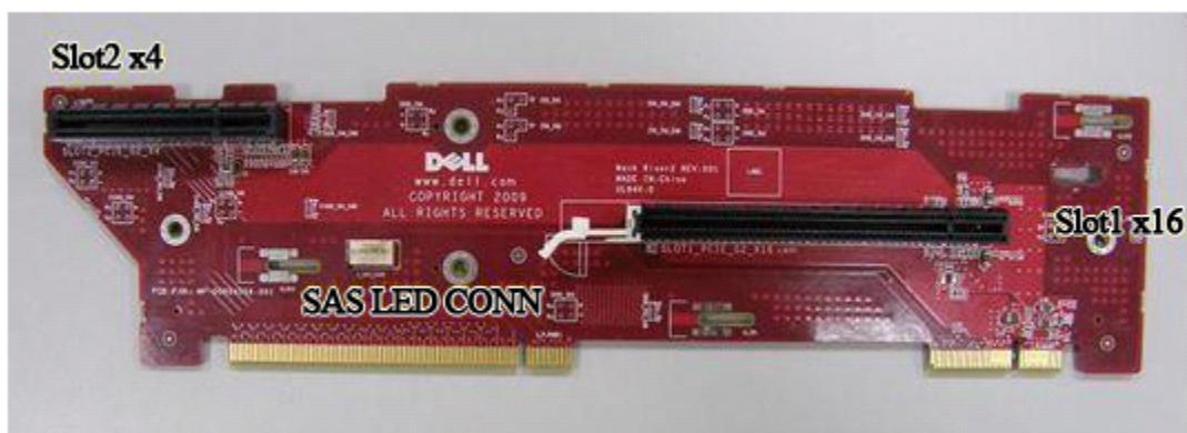
Figure 32. Riser 2
