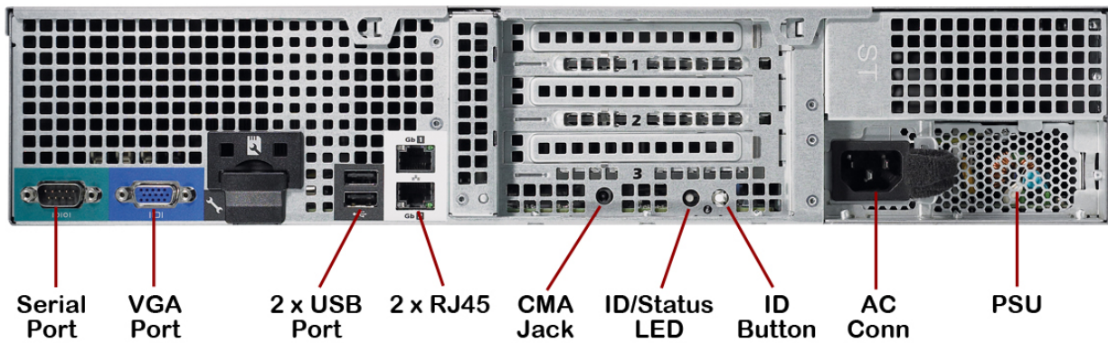
Figure 8. R510 with Non-Redundant Power Supply for PowerEdge R510-4 ONLY
