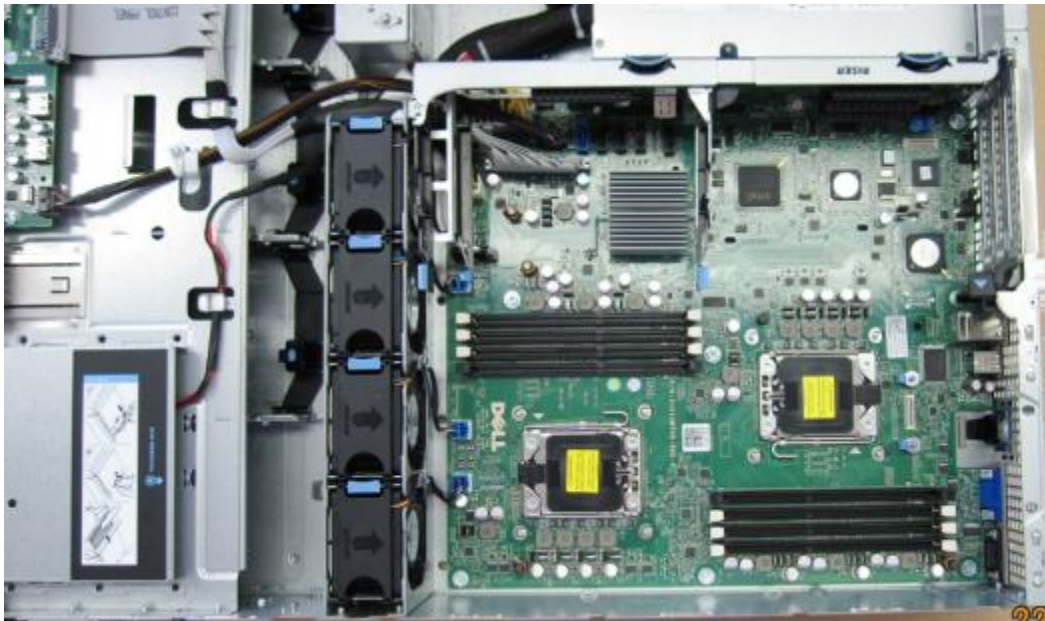
Figure 15. Cabled HDD, No Backplane
