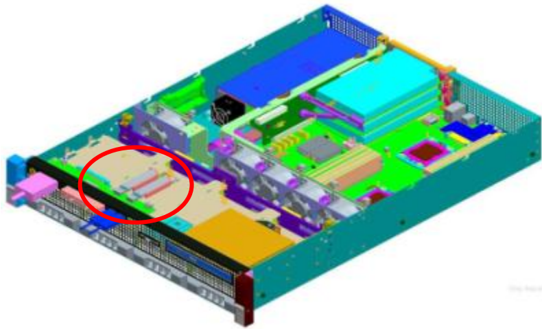
Figure 26. PowerEdge R510-4 Internal USB Connector
