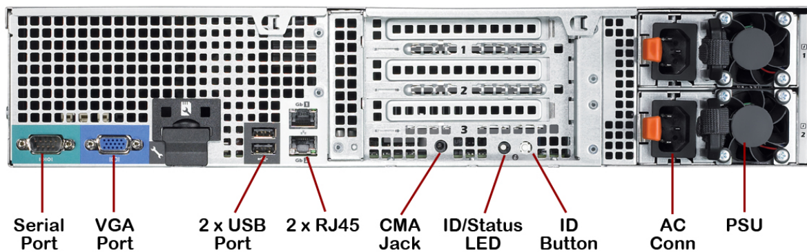
Figure 9. With Redundant Power Supply for PowerEdge R510-8 and 12
