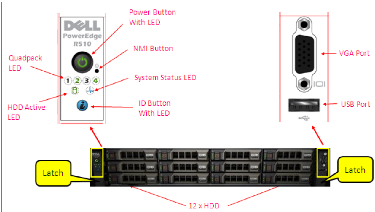
Figure 5. PowerEdge R510-12 HDD Configuration
