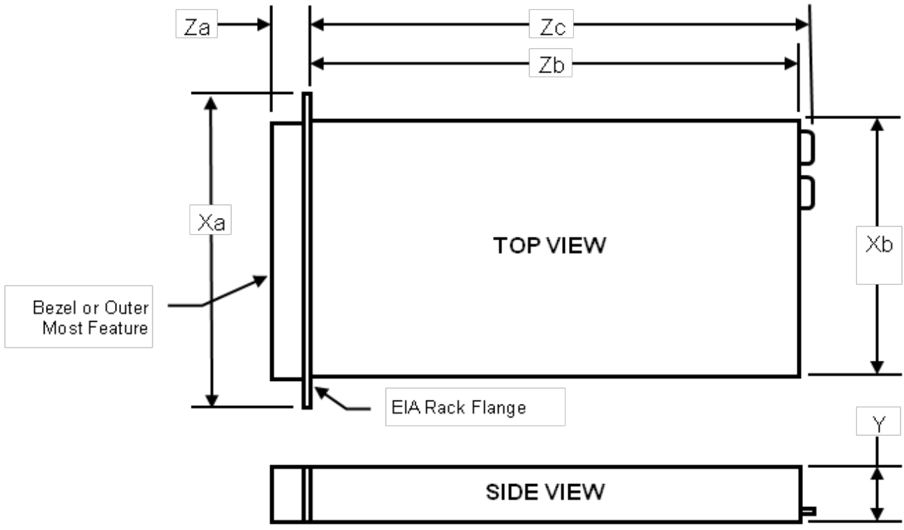
Figure 2. System Dimensions
