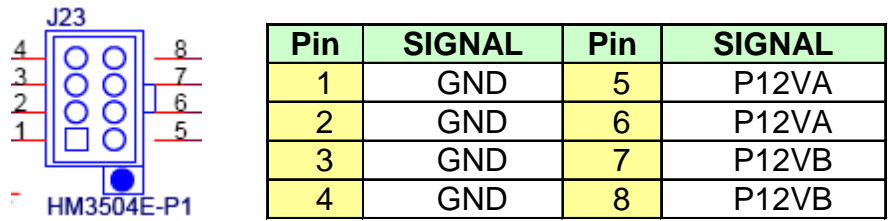
Figure 30. Connector (8 pins)
