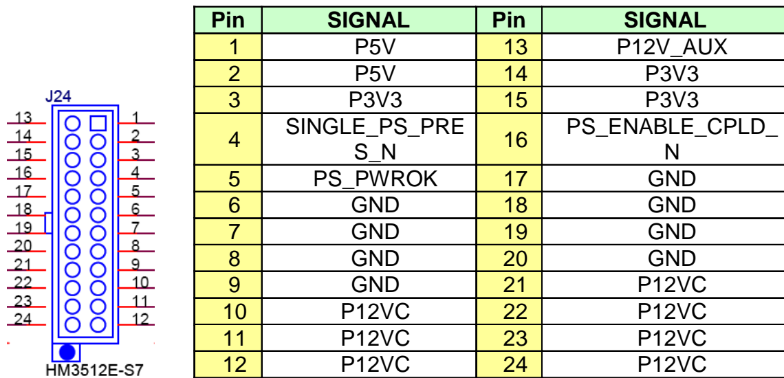
Figure 29. Power Supply Connector (24 pins)
