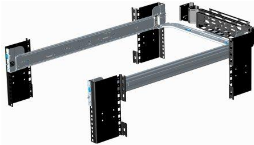
Figure 19. R510 Sliding Rails with CMA
