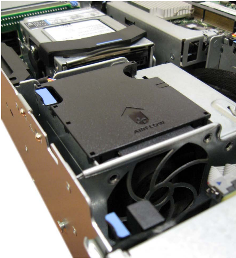
Figure 16. PowerEdge R510-12 Internal View (Redundant PSU with PDB and Additional Fan for PSU)
