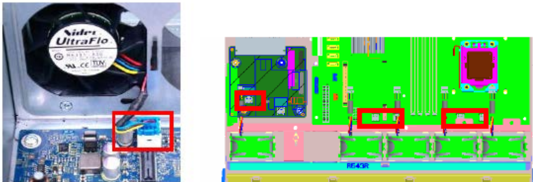
Figure 25. Fan Connector Locations
